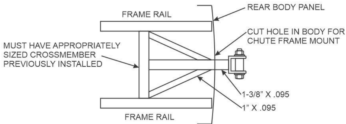
TOP VIEW - 7601
