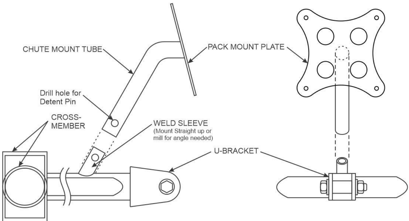
SIDE VIEW - 7601 / 7602
